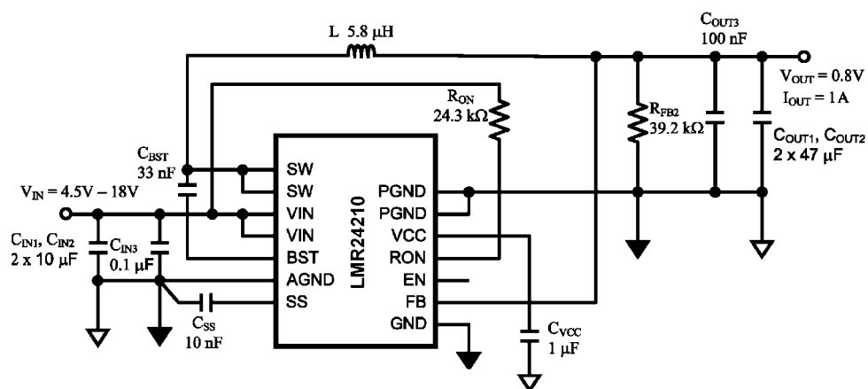
FIGURE 9. Typical Application Schematic for V_{OUT} = 0.8\text{V}
