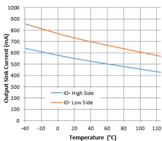
Figure 19. Output Sink Current vs. Temperature
