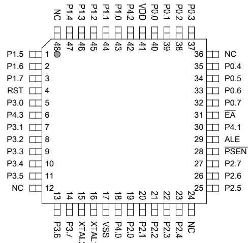
48-pin LQFP
