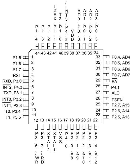
44-pin PQFP
