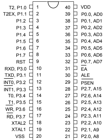
40-pin DIP
