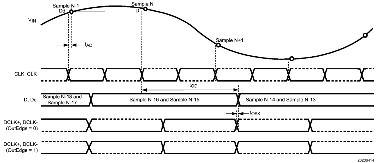
FIGURE 3. ADC08500 Timing — SDR Clocking
