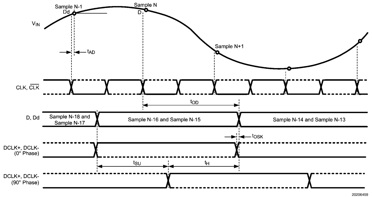
FIGURE 4. ADC08500 Timing — DDR Clocking
