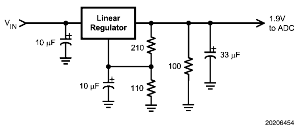
FIGURE 15. Non-Spiking Power Supply
