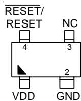
SC-82 (R-Type)
