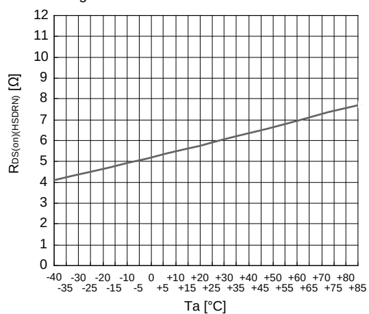
High-side Driver ON resistance vs. Ta
