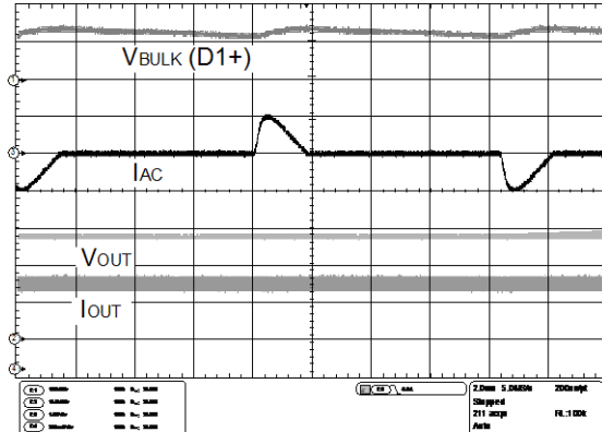
I/O waveform
