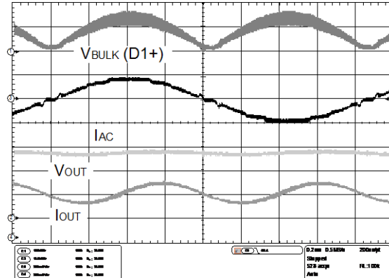
I/O waveform
