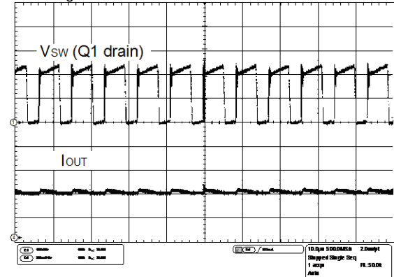
Switching waveform
