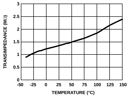
FIGURE 22. TRANSIMPEDANCE vs TEMPERATURE
