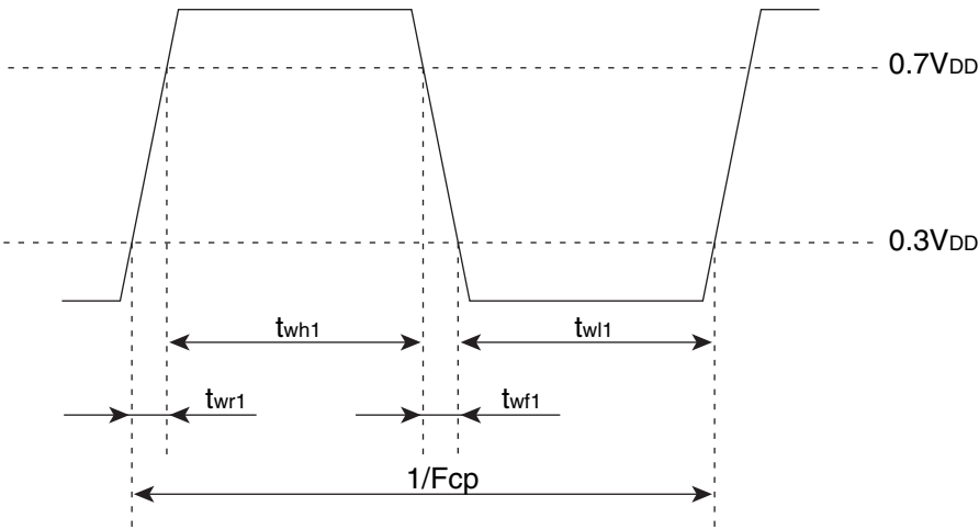
Figure:1.5.2 OSCI Timing Chart
