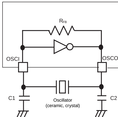
Figure:1.5.1 Oscillation
