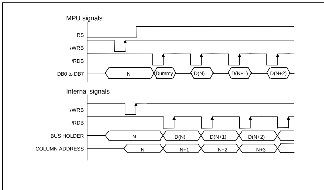
Figure 5. Read Timing
