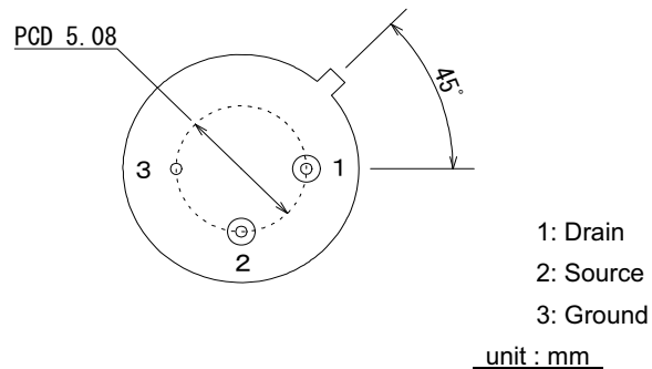
Figure 7. ZSBG446671 Mechanical Configuration
