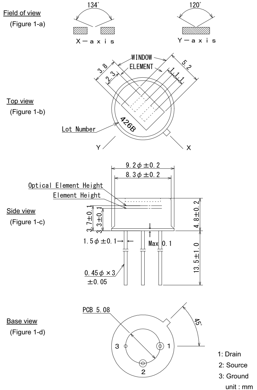
Figure 4. ZSBG323671 Mechanical Configuration
