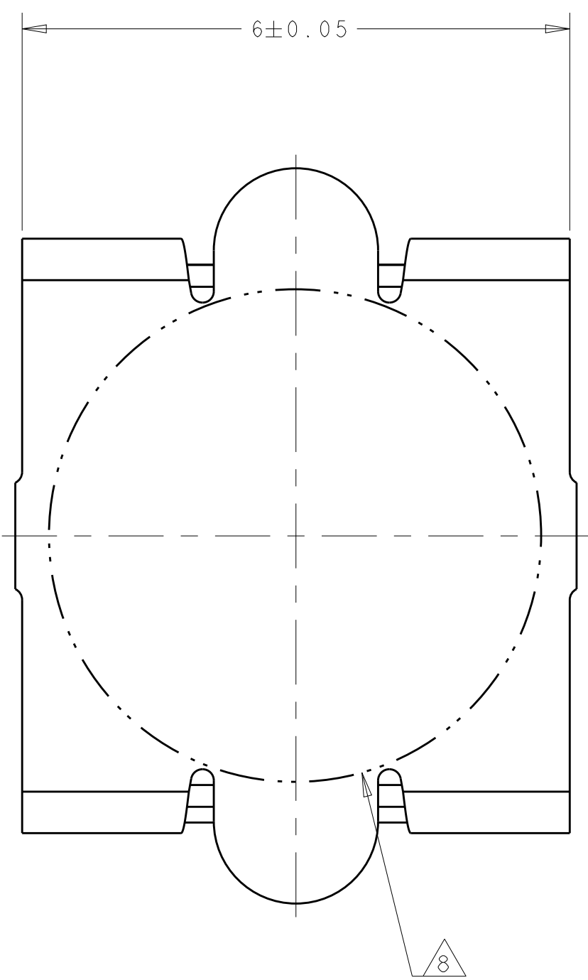
VACUUM COVER
