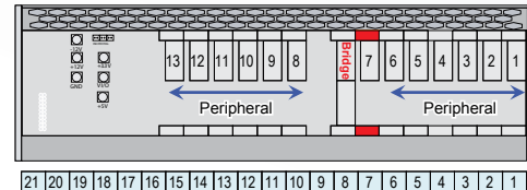
cPCIS-2633R/cPCIS-2833R Inside Rear View
