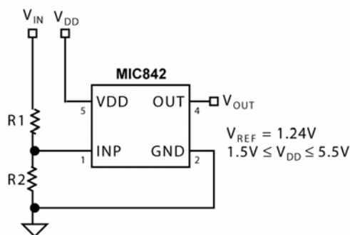
Threshold Detector with Internal Fixed Hysteresis
