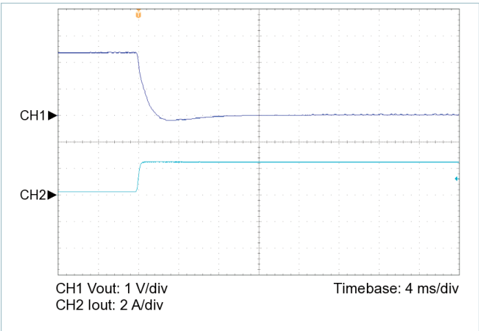
Figure 20 — 10% to 100% load transient response, V_{IN} = 100\text{ V} , nominal trim, C_{OUT\_EXT} = 220\text{ }\mu\text{F}
