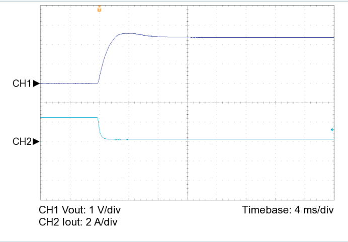
Figure 19 — 100% to 10% load transient response, V_{IN} = 100\text{ V} , nominal trim, C_{OUT\_EXT} = 220\text{ }\mu\text{F}
