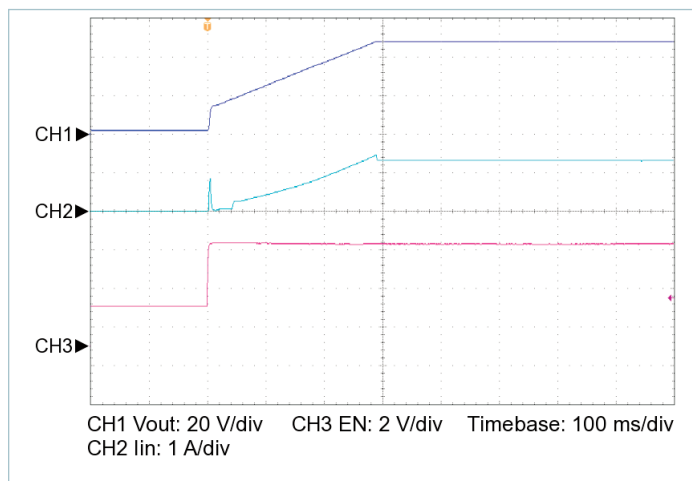
Figure 16 — Startup from EN, V_{IN} = 100\text{ V} , C_{OUT\_EXT} = 2200\text{ }\mu\text{F} , R_{LOAD} = 19.200\text{ }\Omega
