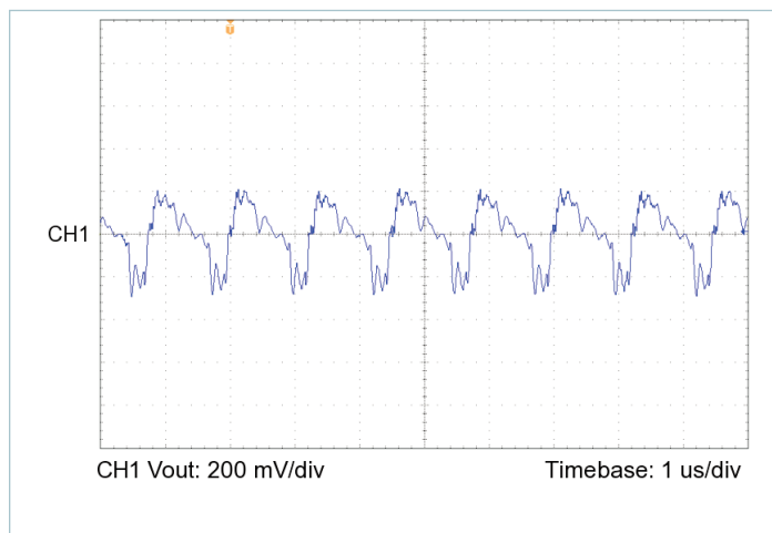
Figure 15 — Output voltage ripple, V_{IN} = 100\text{ V} , V_{OUT} = 48.0\text{ V} , C_{OUT\_EXT} = 220\text{ }\mu\text{F} , R_{LOAD} = 19.200\text{ }\Omega
