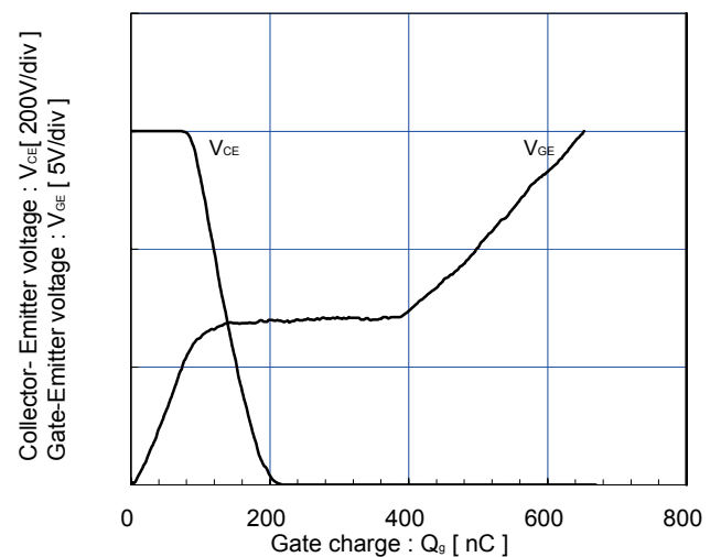
Dynamic Gate charge (typ.) V_{CC}=600\text{V} , I_C=300\text{A} , T_j=25^\circ\text{C}
