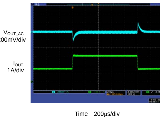
Figure 11. Load Transient ( I_{OUT}=1.5\text{A} to 3\text{A} )
