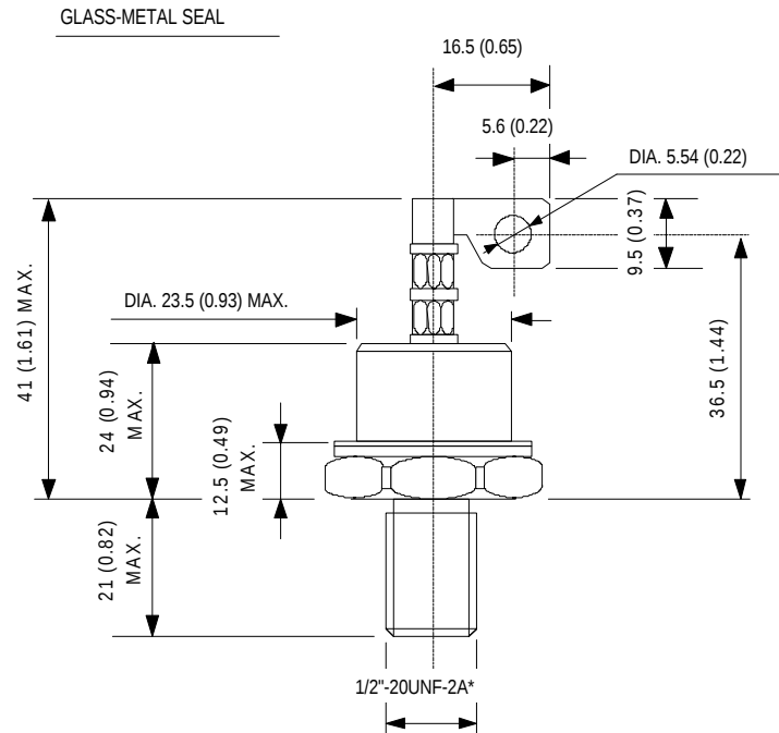
DO-205AC (DO-30) Flag All dimensions in millimeters (inches)
