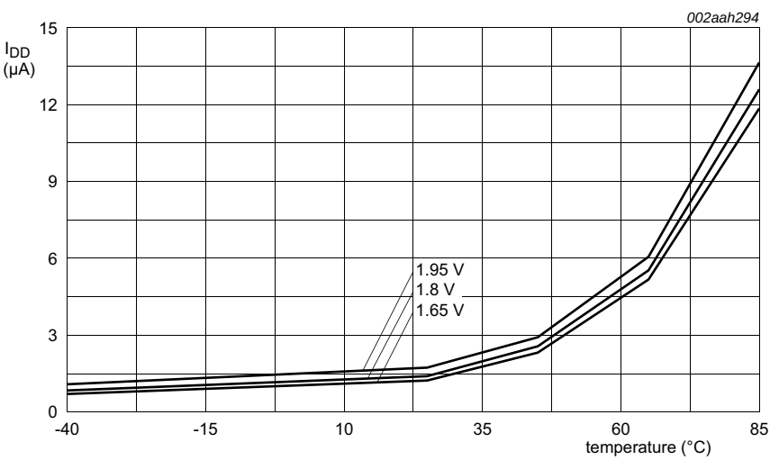
Fig 21. Deep-sleep mode: Typical supply current I_{DD} versus temperature
