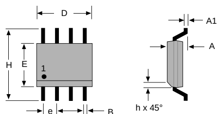
HMC1021S—8-Pin SOIC
