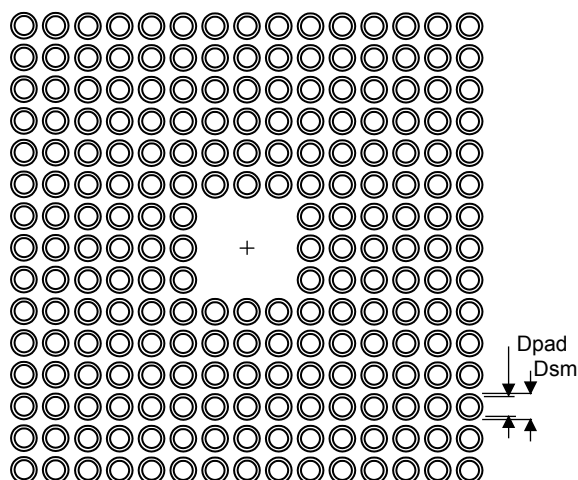
Figure 101. TFBGA216 - Recommended footprint
