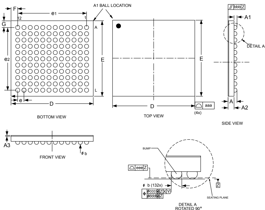
Figure 91. WLCSP132 - Outline
