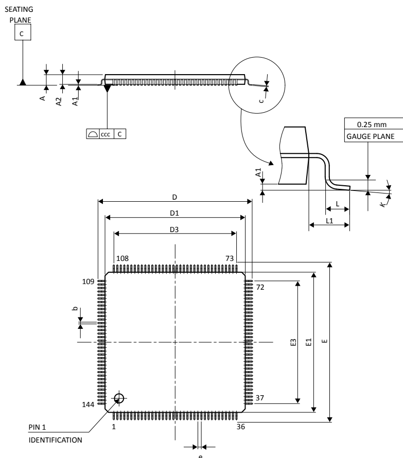
Figure 94. LQFP144 - Outline
