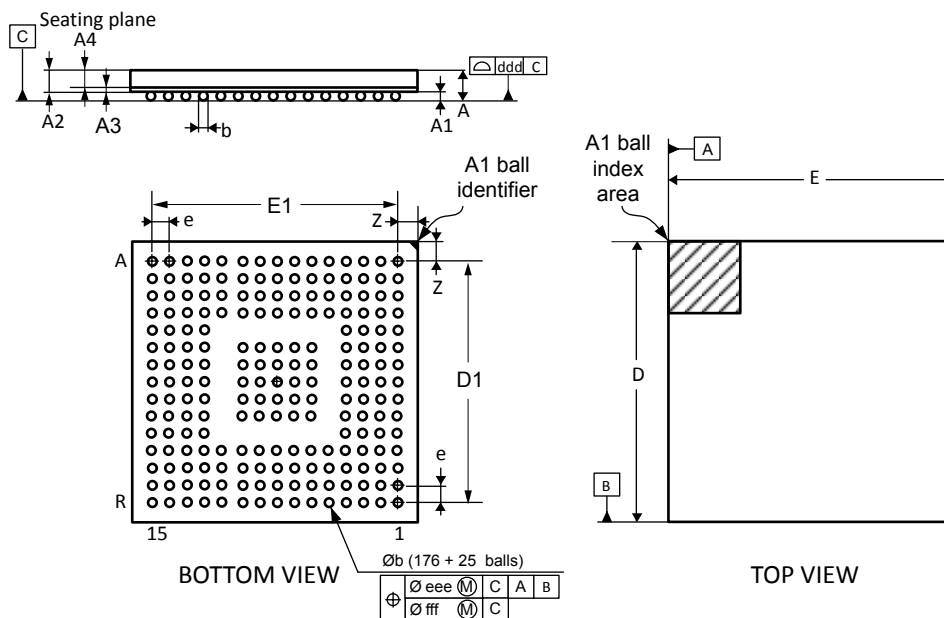
Figure 109. UFBGA176+25 - Outline
