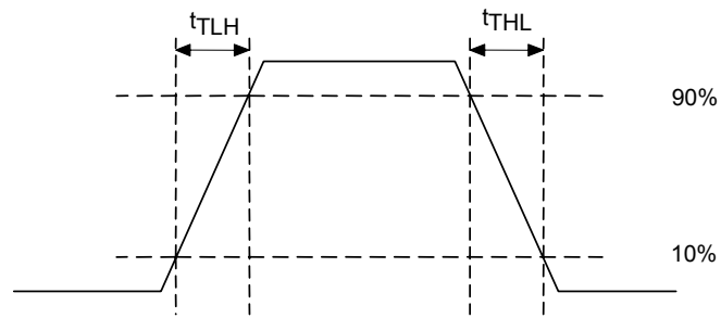
Fig.2 Output transition time measurement conditions
