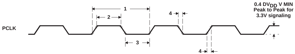
Figure 47. PCLK Timing
