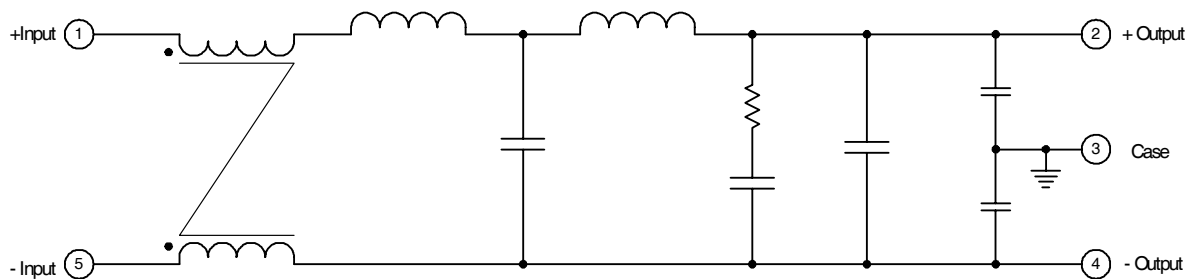
AMH461 Block Diagram
