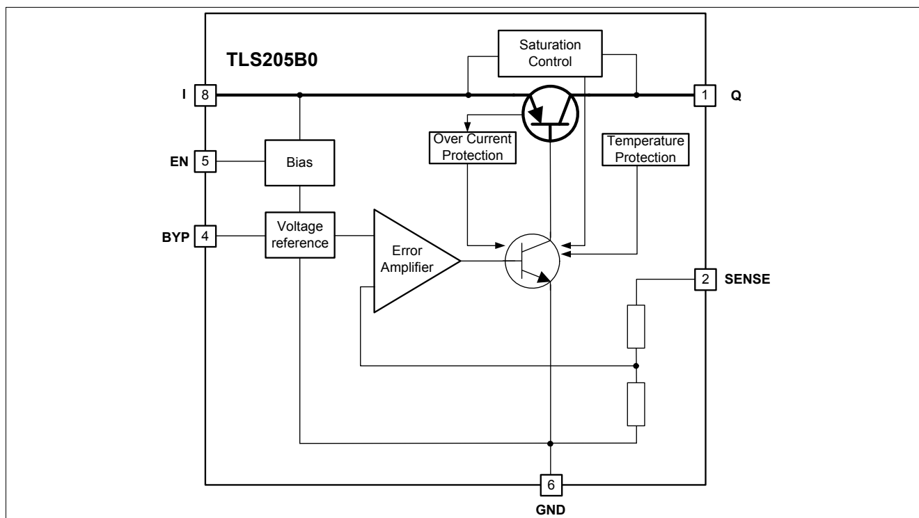
Figure 1 Block Diagram TLS205B0 V33 fixed voltage version
