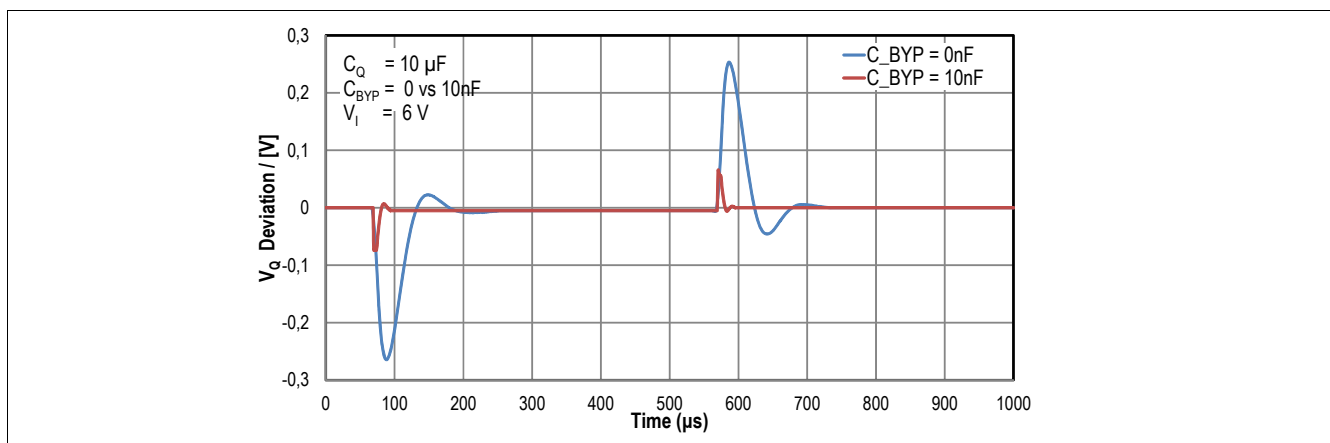
Figure 8 Influence of C_{\text{BYP}} : example of transient response to one and the same load step with and without C_{\text{BYP}} of 10 nF ( I_Q : 100 mA to 500 mA, TLS205B0EJV33)
