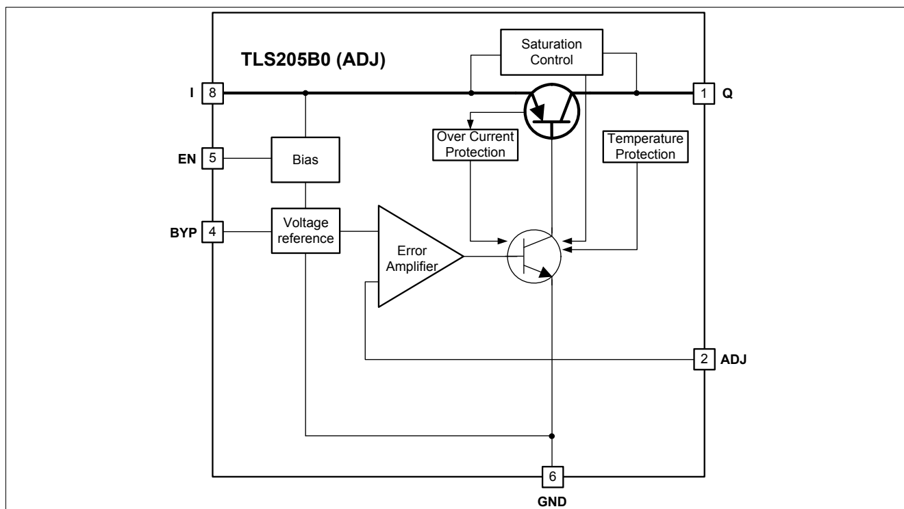
Figure 2 Block Diagram TLS205B0 V adjustable version
