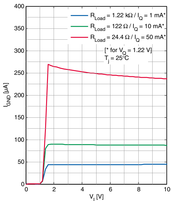
GND Pin Current I_{\text{GND}} versus Input Voltage V_{\text{I}} (TLS205B0EJV)
