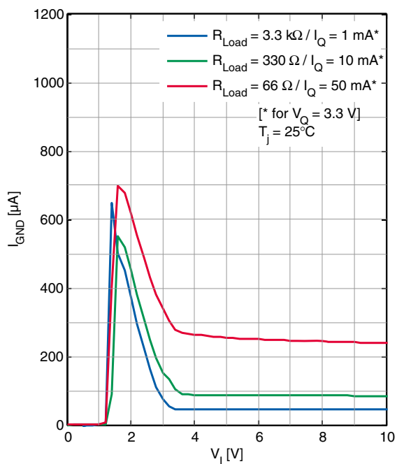
GND Pin Current I_{\text{GND}} versus Input Voltage V_{\text{I}} (TLS205B0EJV33)
