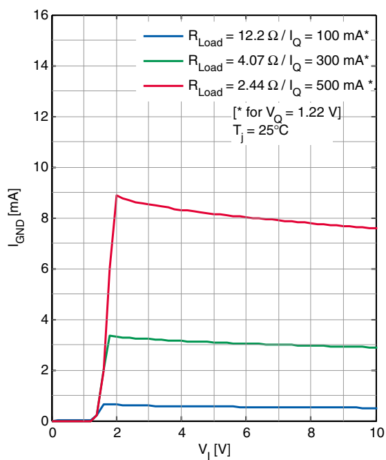
GND Pin Current I_{\text{GND}} versus Input Voltage V_{\text{I}} (TLS205B0EJV)
