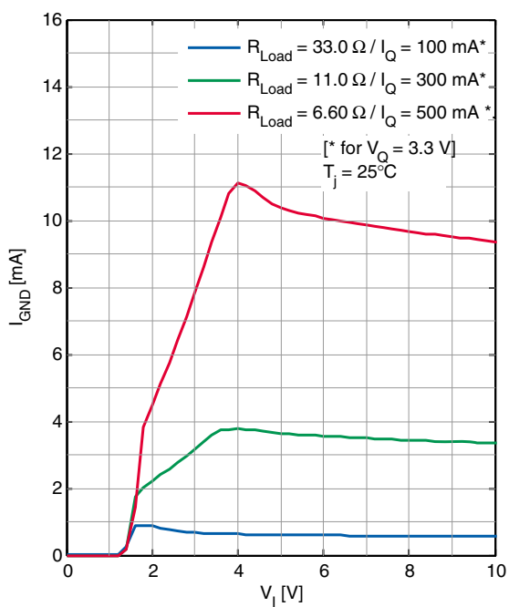
GND Pin Current I_{\text{GND}} versus Input Voltage V_{\text{I}} (TLS205B0EJV33)
