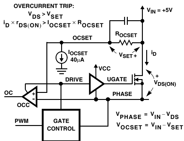
FIGURE 3. OVERCURRENT DETECTION
