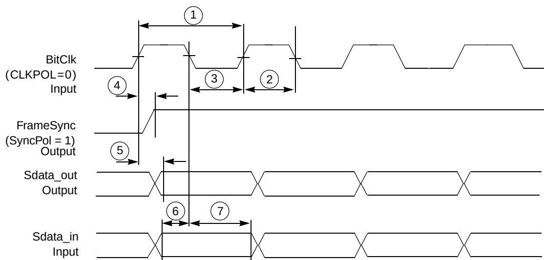
Figure 48. Timing Diagram – AC97 Mode
