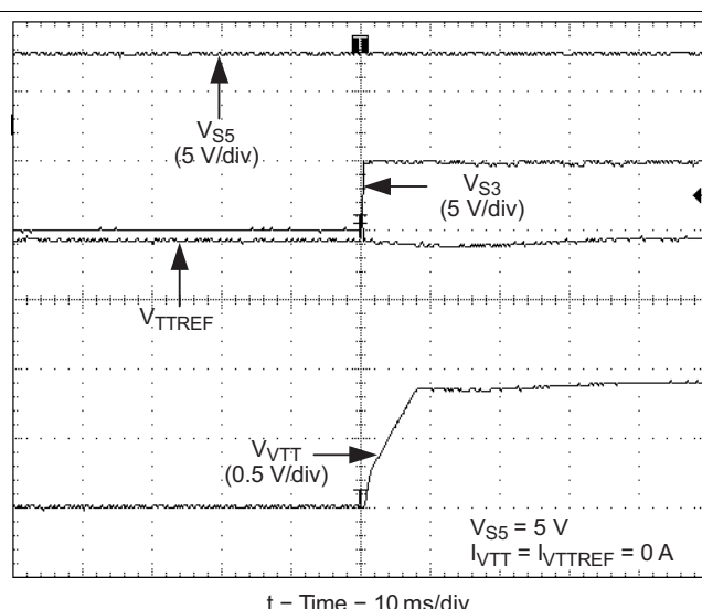
Figure 25. Start-Up Waveforms S3 Low-to-High
