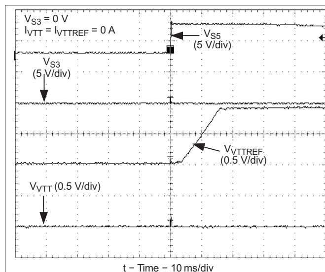
Figure 24. Start-Up Waveforms S5 Low-to-High
