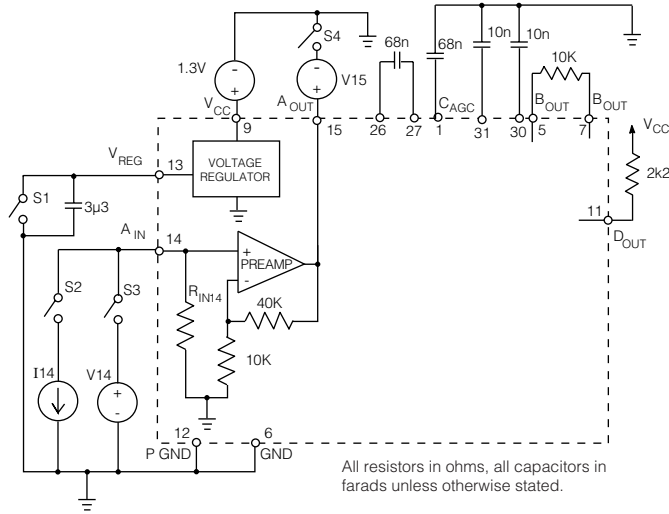
Fig. 1 Preamplifier and Regulator Test Circuit
