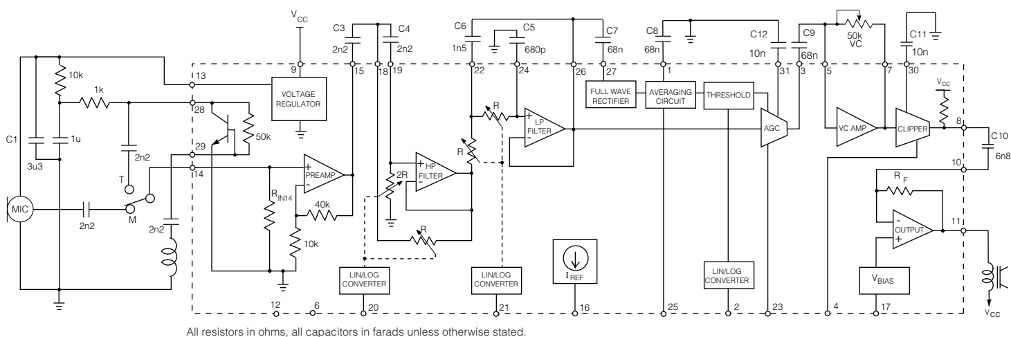
Fig. 16 Typical Telecoil Application Circuit
