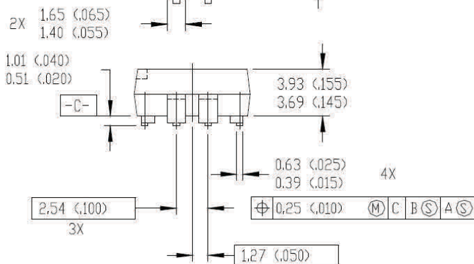
PVI5050NS
