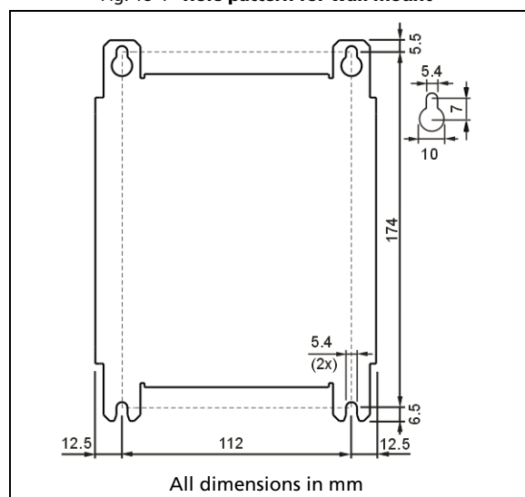
Fig. 18-4 Hole pattern for wall mount
