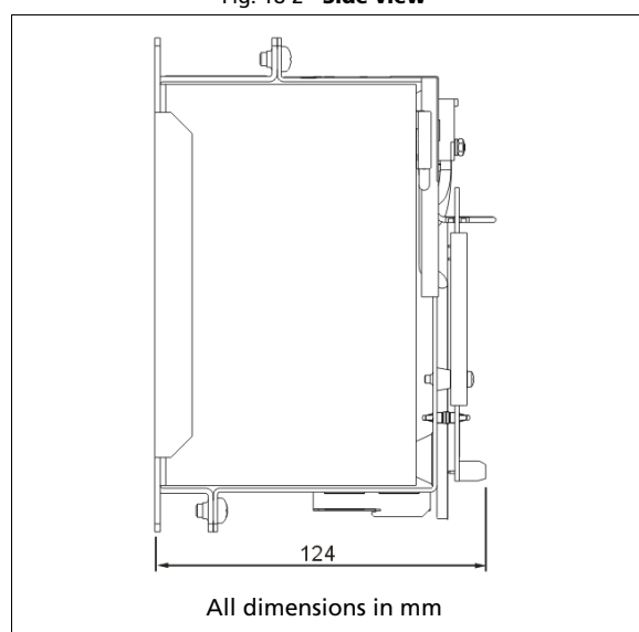
Fig. 18-2 Side view
