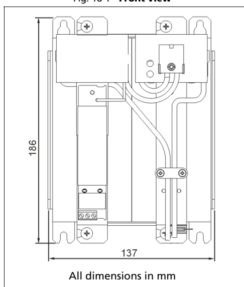
Fig. 18-1 Front view
