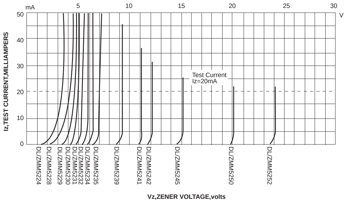
Breakdown characteristics
