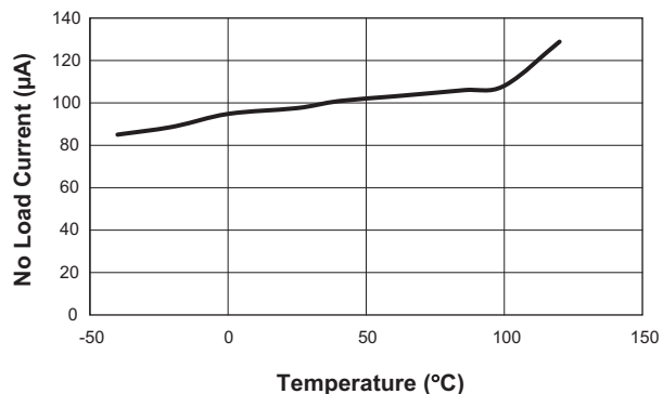
No Load Current vs. Temperature ( V_{IN} = 3.6V ; V_{OUT} = 5.0V )
