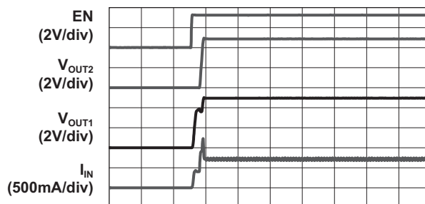
Enable Soft Start ( V_{IN} = 4.2V ; 500mA Load)
