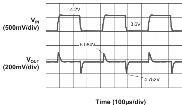
Line Transient Response (16 \Omega Load)
