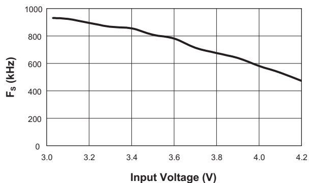
Switching Frequency vs. Input Voltage (24W Load; L = 2.2\mu\text{H} )
