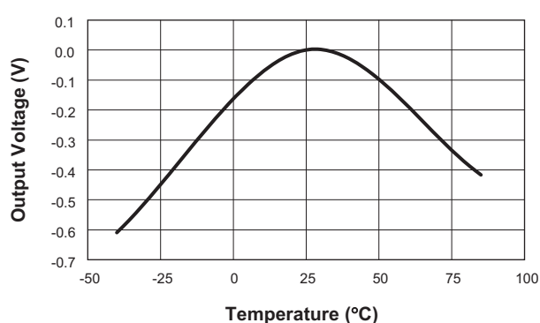
Output Voltage vs. Temperature ( V_{IN} = 3.6V ; 50\Omega Load)
