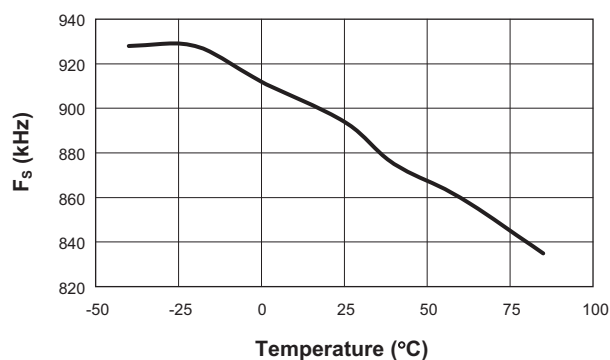
Switching Frequency vs. Temperature ( V_{IN} = 3.6\text{V} ; 16.5 \Omega Load; L = 2.2\mu\text{H} )
