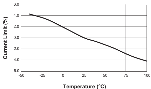
Current Limit vs. Temperature ( R_{SET} = 20.3\text{k}\Omega )
