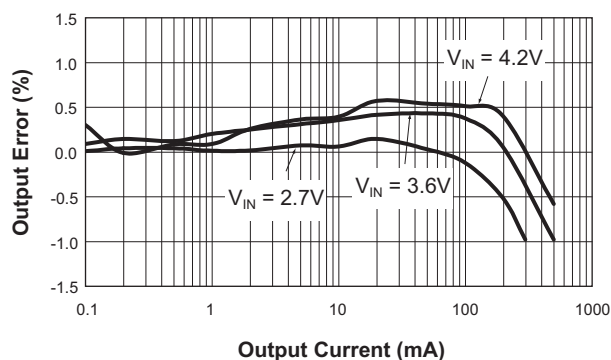
DC Regulation ( V_{OUT} = 5.0V )
