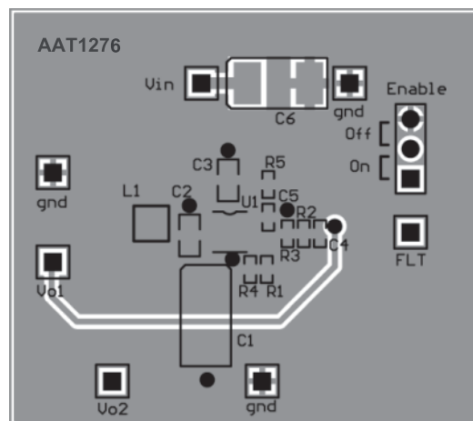
Figure 2: AAT1276 Evaluation Board Bottom Side Layout.
