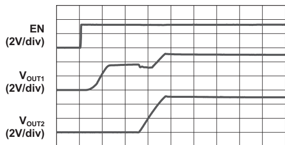
Enable Soft Start ( V_{IN} = 3.6V ; C_{VOUT2} = 120\mu F ; 16 \Omega Load)
