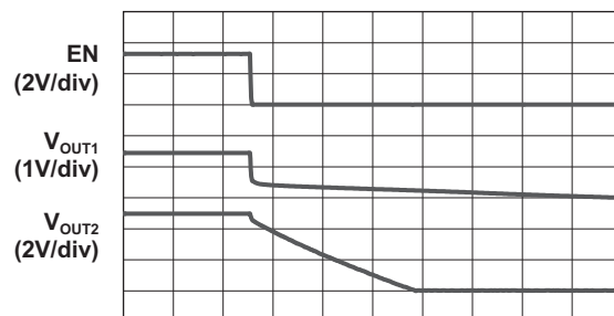
Shutdown ( V_{IN} = 3.6V ; C_{VOUT2} = 120\mu F ; 16 \Omega Load)
