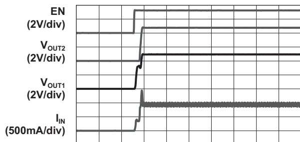
Enable Soft Start ( V_{IN} = 3.6V ; 500mA Load)
