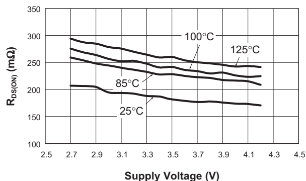
N-Channel R_{DS(ON)} vs. Supply Voltage
