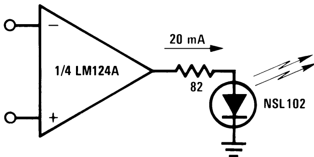
Figure 17. DC Summing Amplifier (V_{\text{IN'S}} \geq 0\text{ V}_{\text{DC}} \text{ And } V_O \geq V_{\text{DC}})
