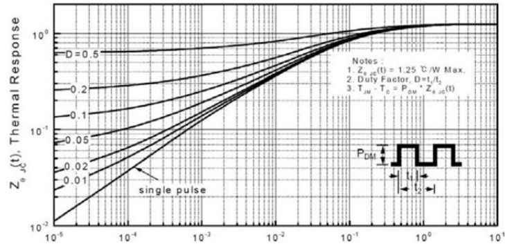
Fig. 10 Transient Thermal Response Curve(ITO-220)
