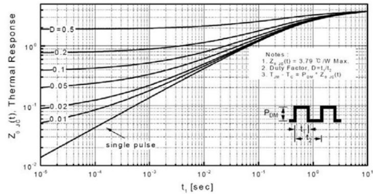
Fig. 11 Transient Thermal Response Curve(TO-220AB)
