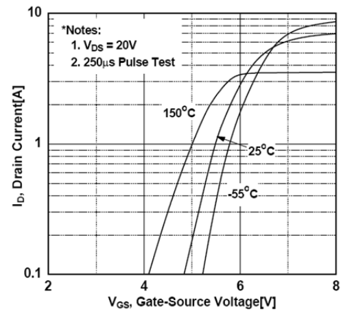
Fig. 2 Transfer Characteristics
