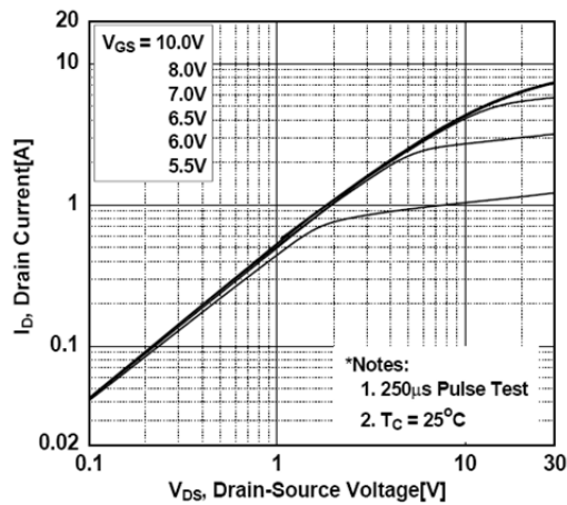
Fig. 1 On-State Characteristics
