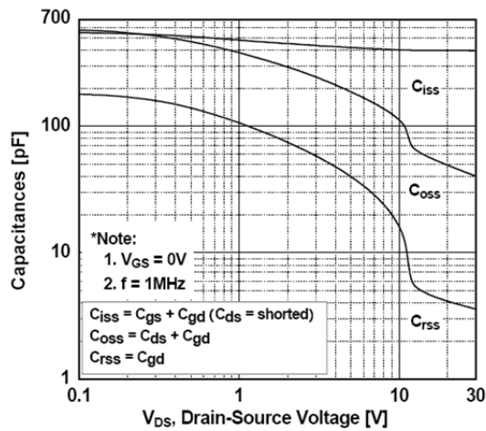
Fig. 5 Capacitance Characteristics
