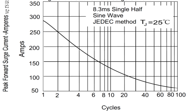
Figure .3-Peak Forward Surge Current
