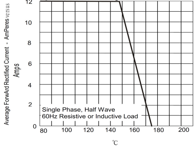
Figure .2- Forward Derating Curve
