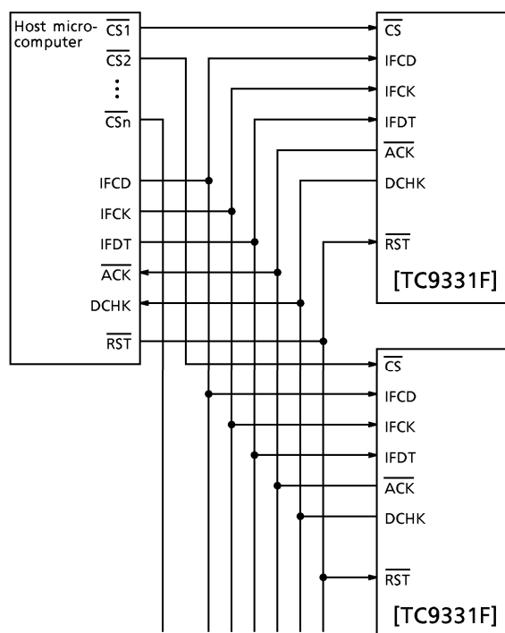
Fig.9 The relationship between the host microcomputer and the TC9331F
