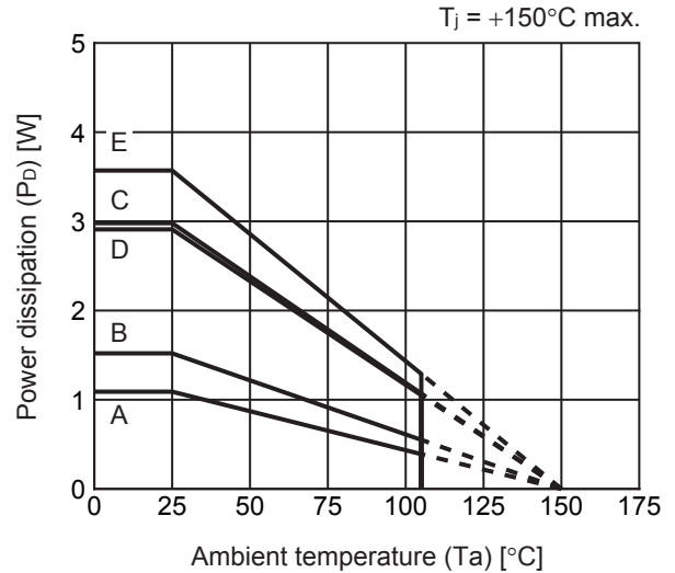
HSOP-8A
