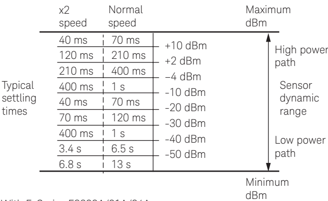
With E-Series E9300A/01A/04A sensors
