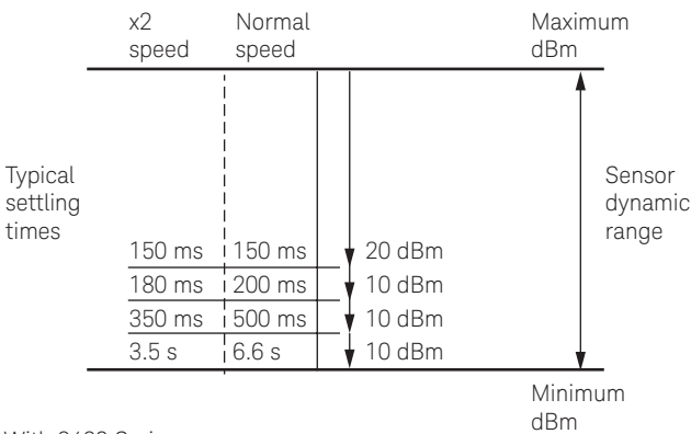
With 8480 Series sensors
