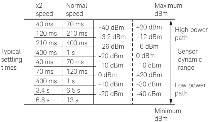
With E-Series E9300B/01B/00H/01H sensor
