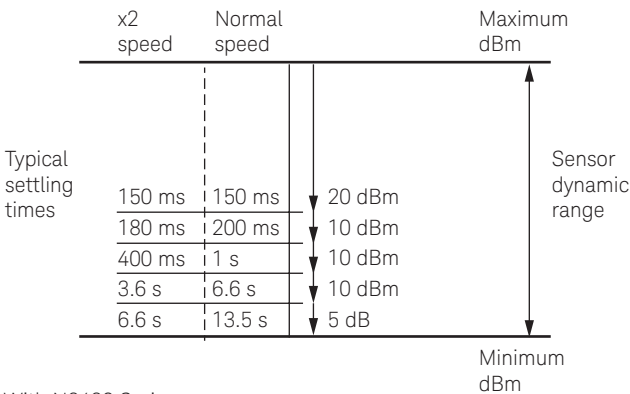
With N8480 Series sensors
