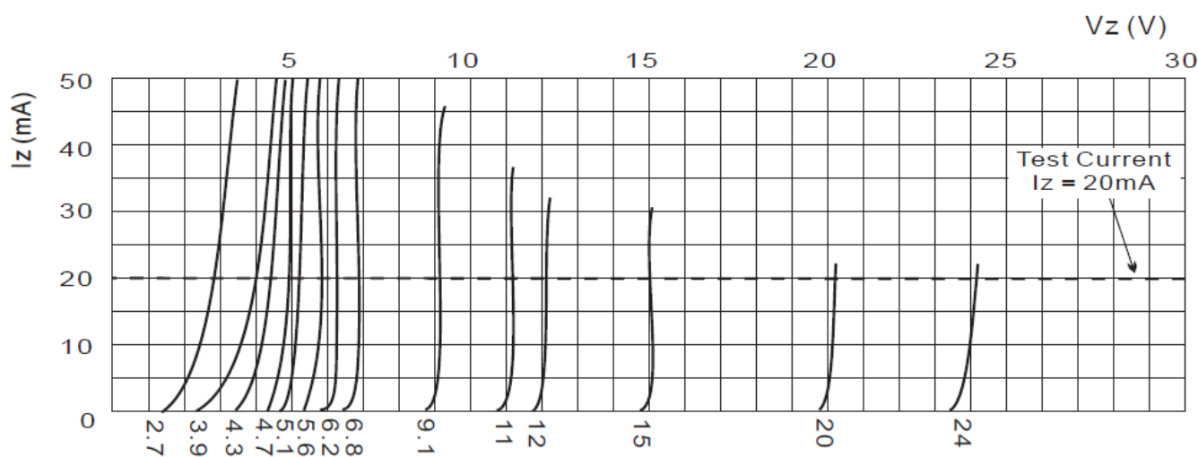
Fig.2 Breakdown Characteristics
