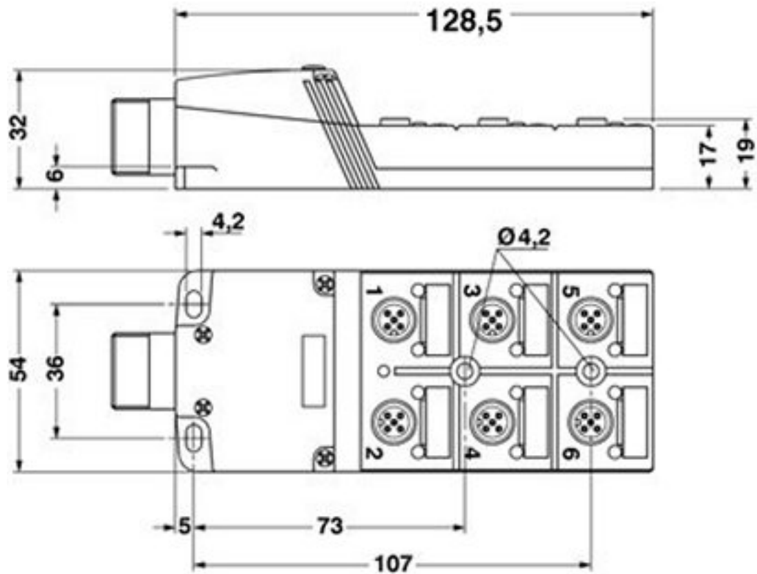
Dimensioned drawing
