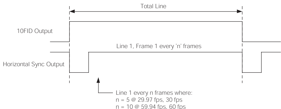
Figure 3-6: Default 10FID Output Timing
