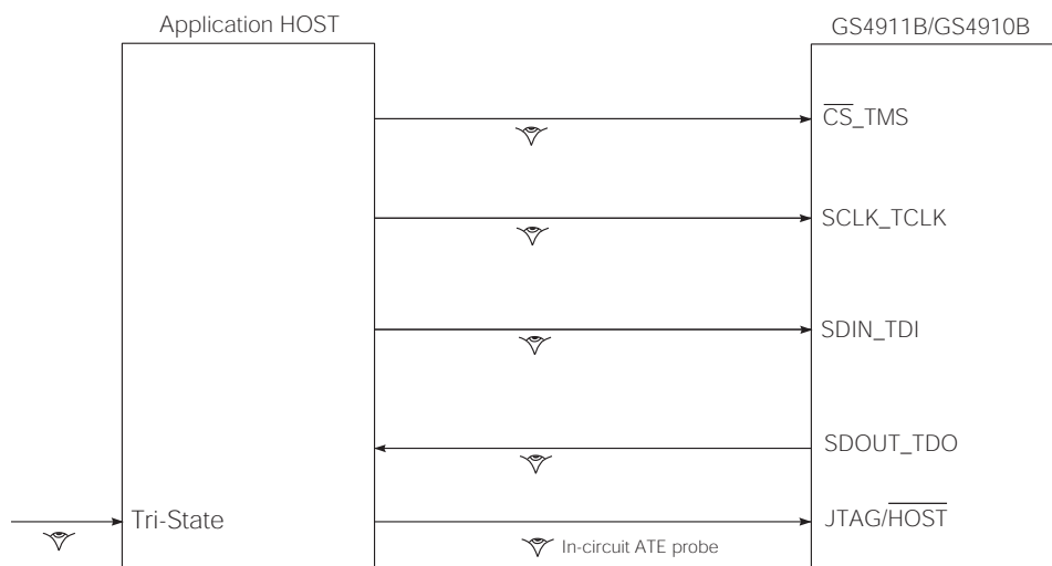
Figure 3-17: System JTAG
