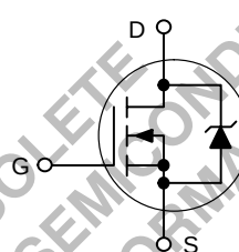
N-Channel
