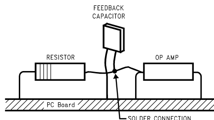
Figure 29. Air Wiring
