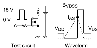
Fig. 8.15 Test Circuit/Waveform
