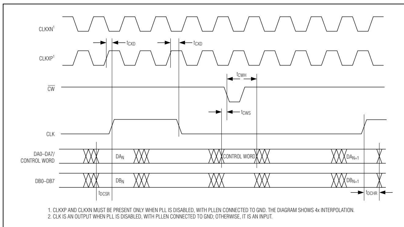
Figure 6. Timing Diagram for Noninterleave Data Mode ( IDE = \text{Low} )
