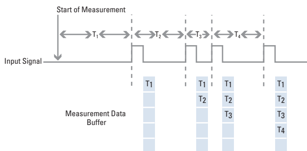
Figure 1. Buffered Period Measurement with Counter/Timers
