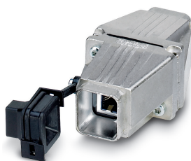
RJ45 push-pull coupling
