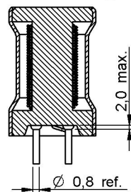
sectional drawing A-A
