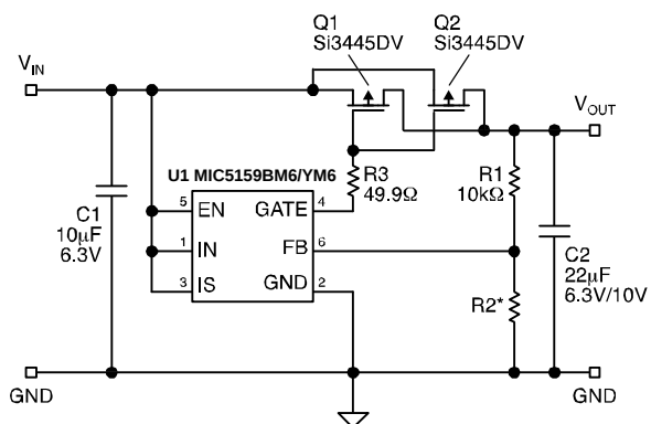
Application Circuit
