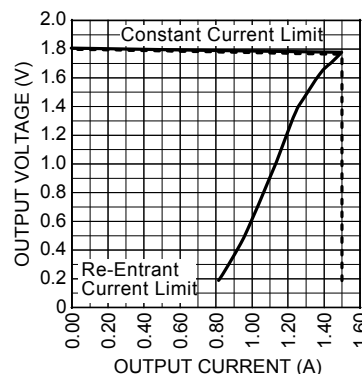
Figure 2. Output Voltage Characteristics Re-Entrant Current Limit
