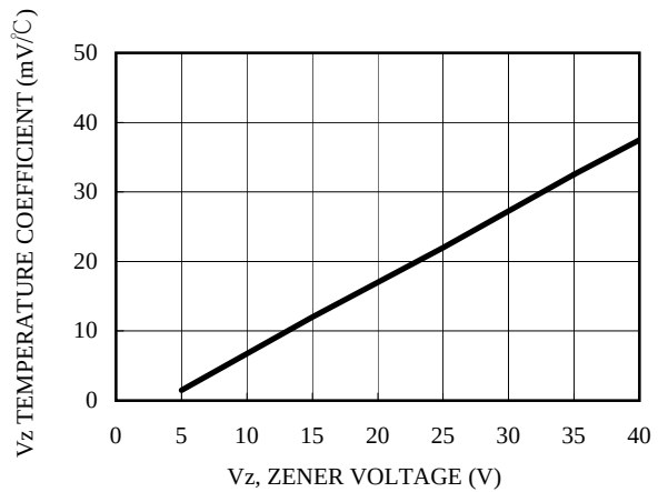
FIG. 2-TYPICAL TEMPERATURE COEFFICIENTS
